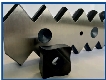
Untha knife and counterknife
